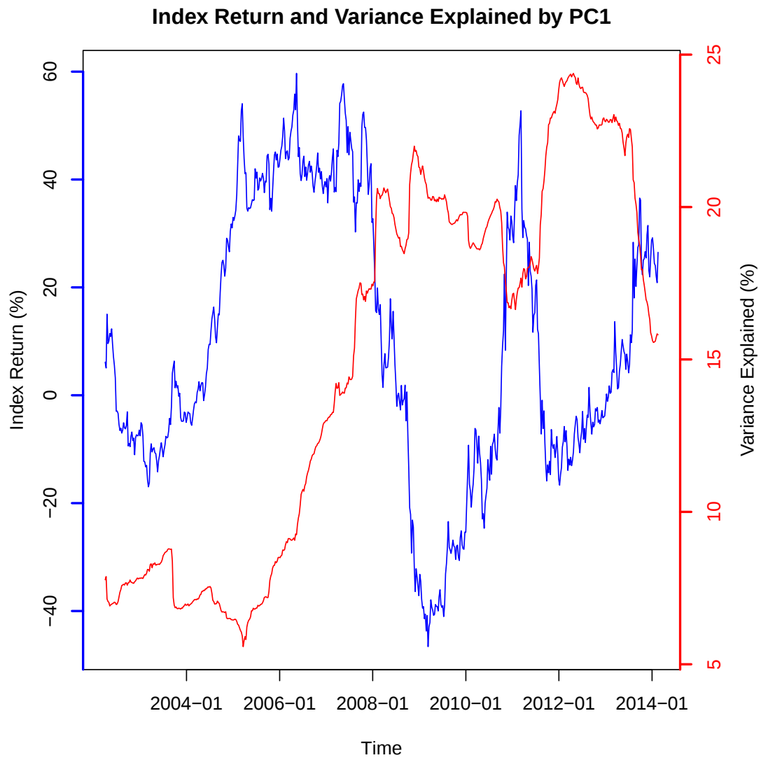
Figure 3: Variance explained by PC1 and the ASX200 index returns. Both the variance explained by PC1 and the ASX200 index returns were calculated weekly using a rolling window size of two years (equivalent to 504 trading days).
