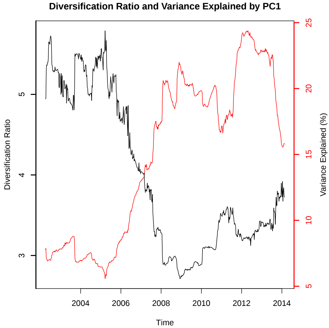
Figure 5: Variance explained by PC1 and the diversification ratio. The variance explained by PC1 was calculated weekly using a rolling window size of two years (equivalent to 504 trading days). The diversification ratio was calculated using Equation (1).
