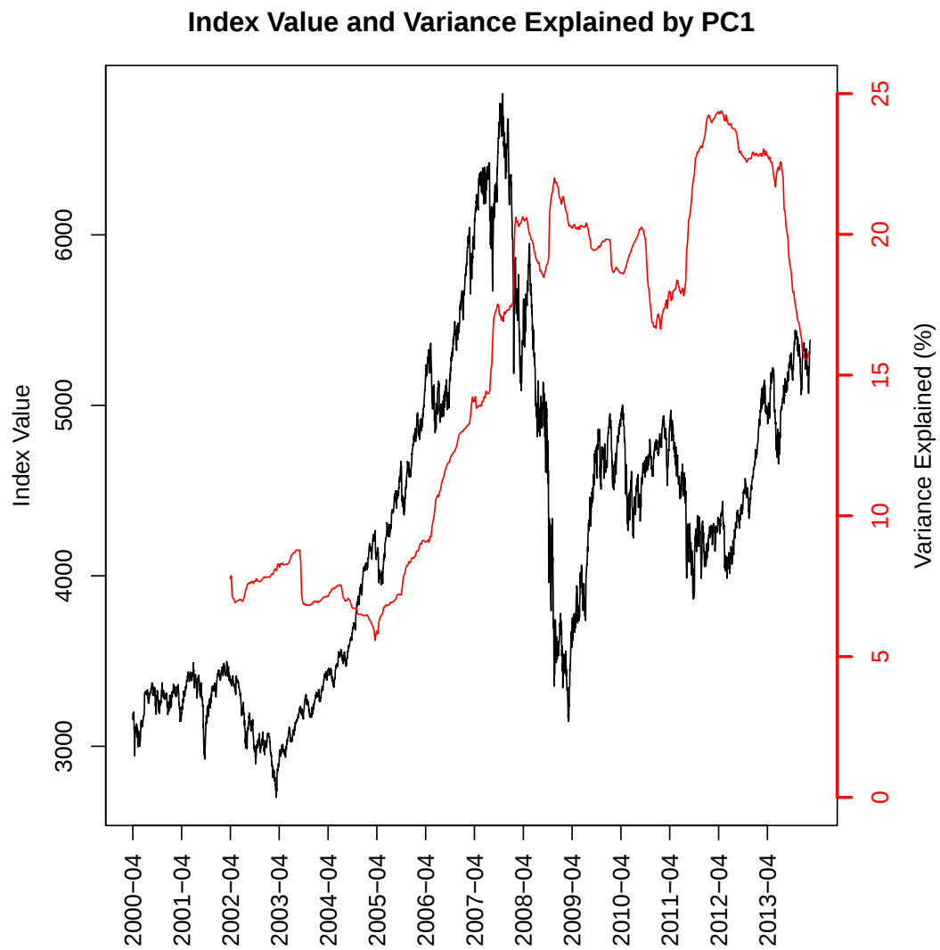
Figure 2: Variance explained by PC1 with the ASX200 index value. The plot of index values includes the first two year period used for the estimation of the PCA.
