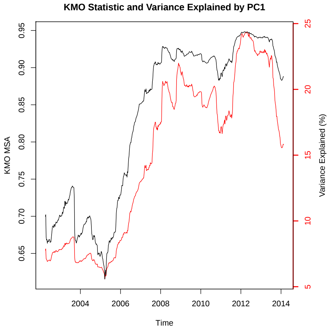
Figure 1: KMO measure of sampling adequacy for 156 stocks and the variance explained by PC1. Both measures were calculated weekly using a rolling window approach with window size two years (504 trading days).
